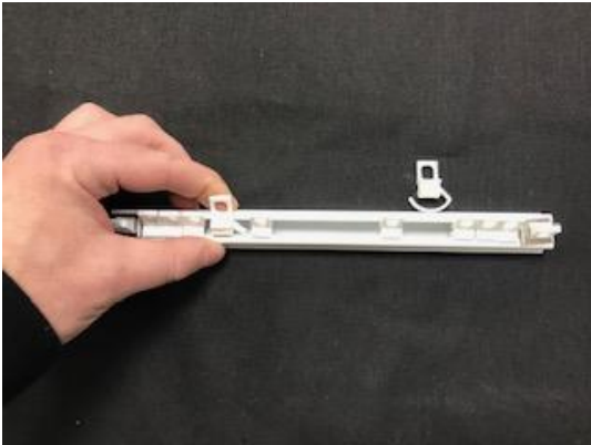
IMAGE 12 (780002 STOP CARRIER)
